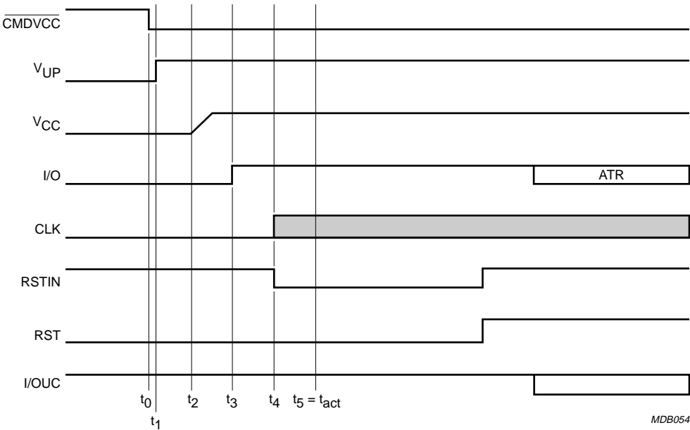
Fig.5 Activation sequence using RSTIN and \overline{\text{CMDVCC}} .
