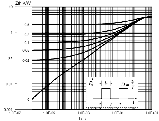
Fig. 12. Transient thermal impedance.
